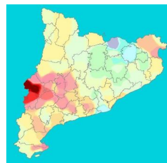
Fig. 5 Accumulated drought (Drought Code Index) of 07/27/08.
